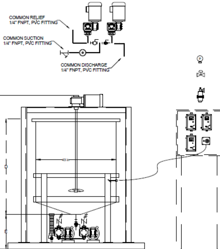
VISUAL REFERENCE - PUMPS INSTALLED UNDER TANK
