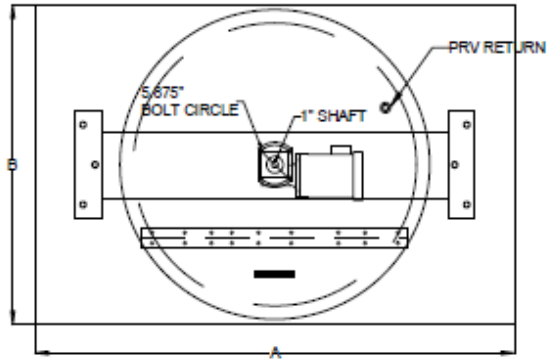
VISUAL REFERENCE - PUMPS INSTALLED UNDER TANK
